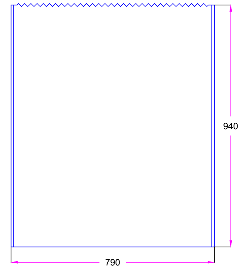
Block E678/B1 Front View
