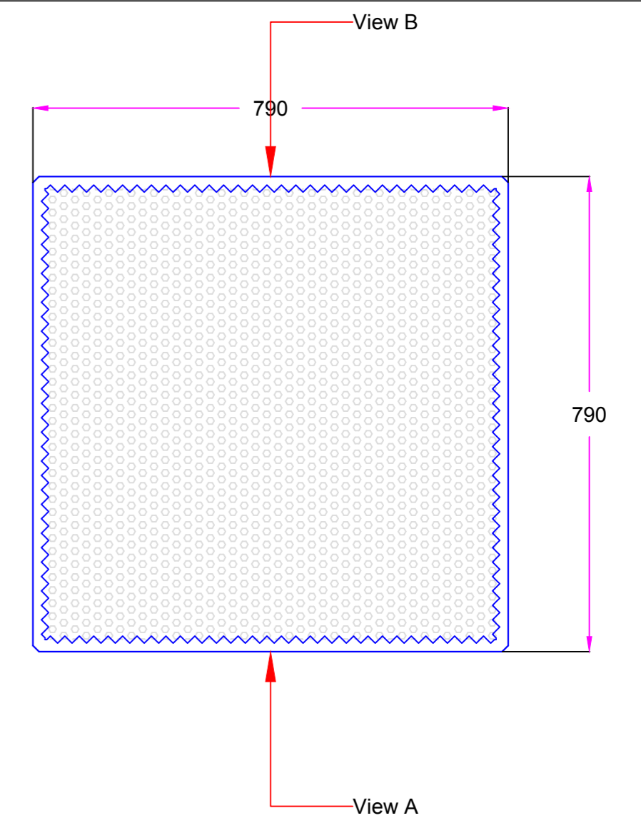
Block E678/B1 Top View
