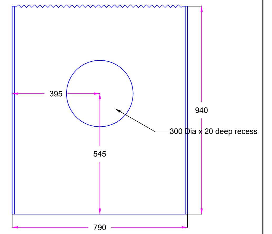
Block E678/B2 View A and View B
