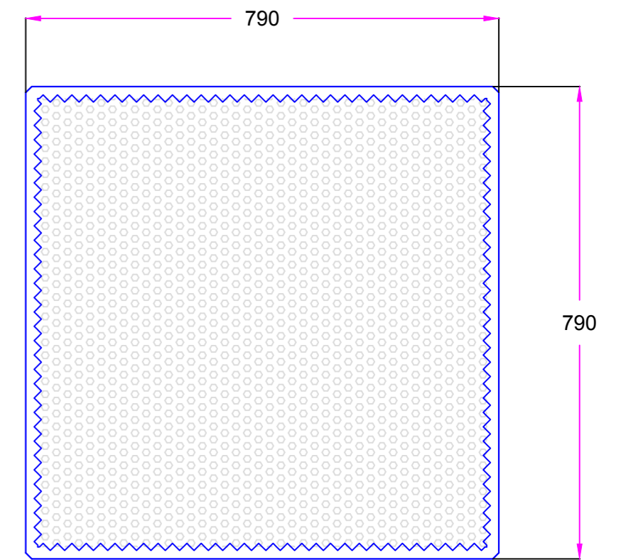
Block E678/B1 Top View
